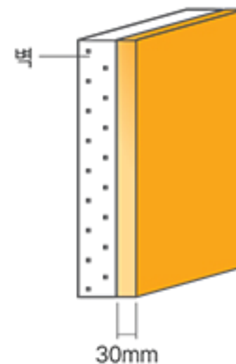
VIP(0.0045W/mk) 적용
