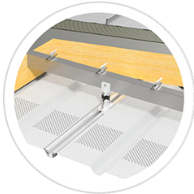
PR PANEL
